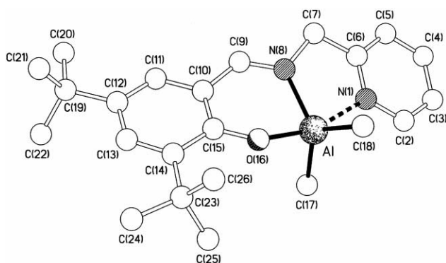
Fig. 4 The molecular structure of 2c .
