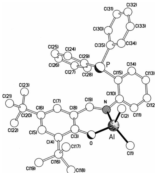
Fig. 5 The molecular structure of 2e showing the tetrahedral geometry at aluminium and the non-coordination of the phosphorus centre.
