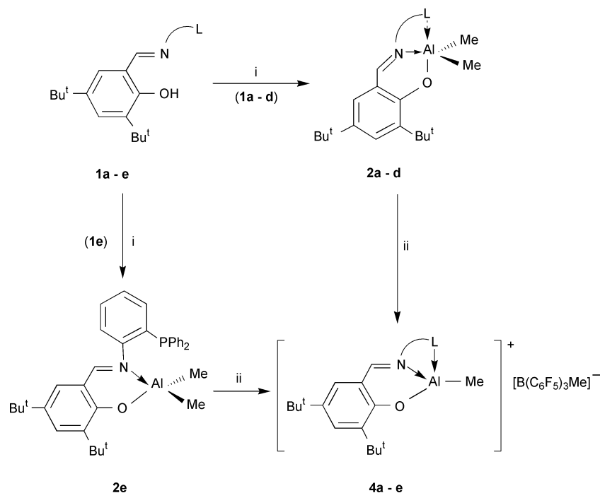
Scheme 1 Formation of aluminium complexes 2a–e and corresponding cations 4a–e . Reagents: i. \text{AlMe}_3 , toluene; ii. \text{B}(\text{C}_6\text{F}_5)_3 , \text{C}_6\text{D}_6 or \text{CD}_2\text{Cl}_2 .
