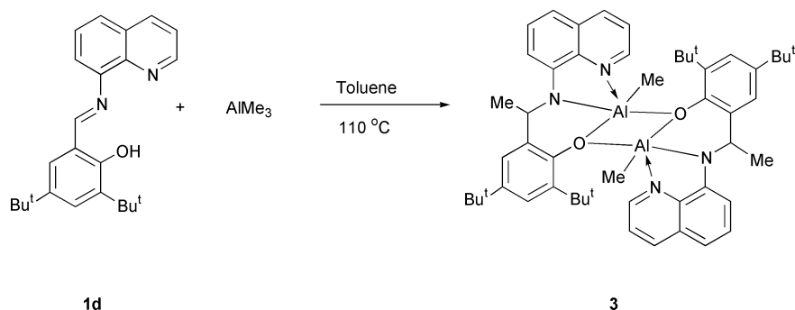
Scheme 2 The preparation of 3 .
