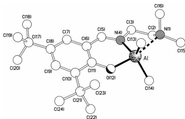
Fig. 3 The molecular structure of 2a , showing the trigonal bipyramidal geometry at aluminium and the very long \text{Al}-\text{N} (amino) linkage.
