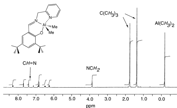
Fig. 2 ^1\text{H} NMR spectrum (250 MHz) of 2c in \text{C}_6\text{D}_6 .
