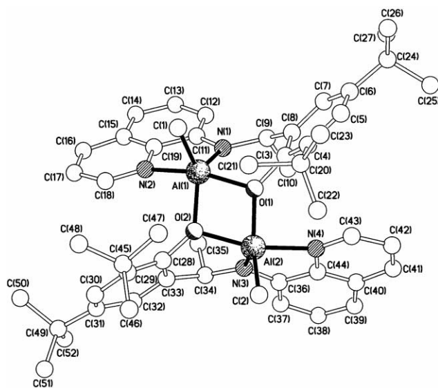
Fig. 6 One of the two independent dimeric molecules present in the structure of 3 .
